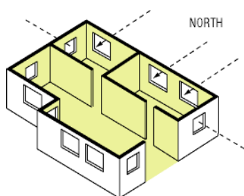
Figure 6.9: Use thermal mass in rooms that may overheat in summer
