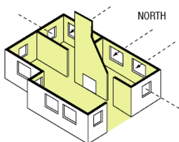
Figure 6.10: Fireplaces on internal walls
