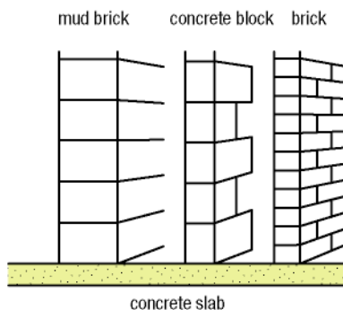
Figure 6.1: Materials with high thermal storage capacity
