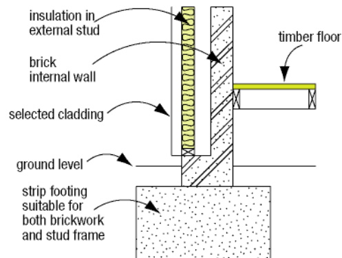
Figure 6.14: Reverse brick veneer with timber floor
