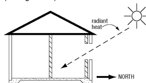
Figure 6.8: Locate thermal mass in north-facing rooms
