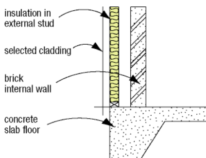
Figure 6.13: Reverse brick veneer on concrete slab
