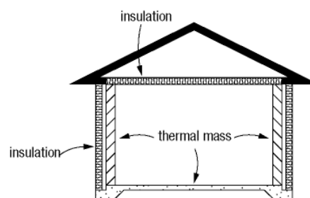
Figure 6.6: Thermal mass within the insulated envelope
