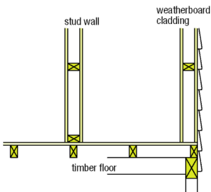
Figure 6.2: Materials with low thermal storage capacity
