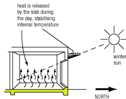
Figure 6.5: Thermal mass in winter
